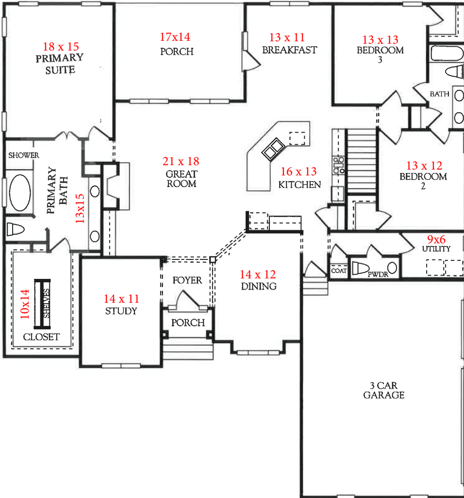
First Floor
